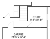
OPTIONAL STUDY REPLACES TANDEM GARAGE
